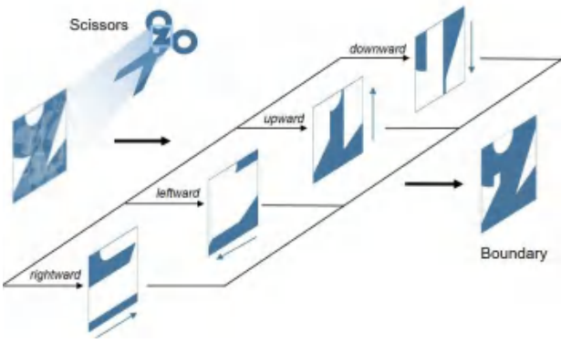
Figure 4. The schematic diagram of Boundary Activation.
